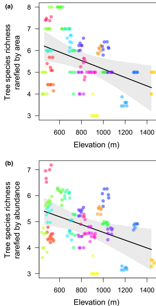
FIGURE 2 Relationships between rarefied species richness and elevation across forest plots in the H. J. Andrews Experimental Forest between 1971 and 2014. (a) Species richness in each census of each forest plot rarefied to 0.25 ha area, the minimum area across forest plots. (b) Species richness in each census of each forest plot rarefied to 51 individuals, which was the minimum abundance across forest plots and censuses. Values of rarefied species richness from the same forest plot (i.e. from different censuses of the same forest plot) have the same colour. The 95% credible interval of the posterior distribution for the slope is shown in grey. Bayesian inference from mixed-effects models that contain random effects of forest plot and census to account for temporal and spatial autocorrelation indicated that slope of the fixed-effects relationship had a 98.2% and 98.6% probability of being less than zero in panels (a) and (b) respectively. Values are slightly adjusted ( \pm 5 –30 m elevation) on the x-axis and points transparent for ease of visualisation
