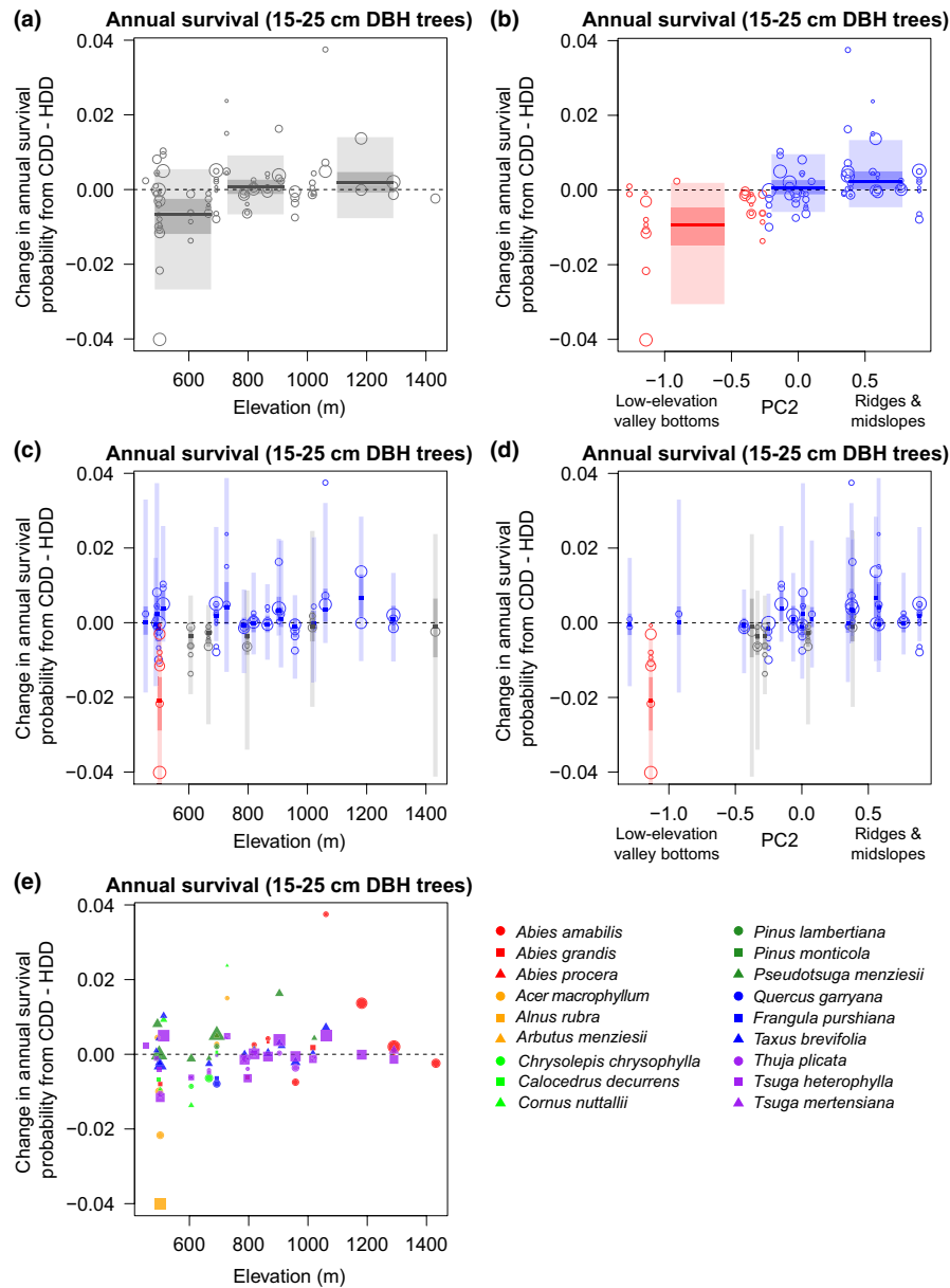
FIGURE 5 Average-predictive comparisons of CDD–HDD in survival of 15–25 cm DBH trees across elevation and microclimate variables ( PC2_{\text{MinSpring}} ). CDD–HDD in survival was defined as the difference in annual survival probability for a focal tree in a stand of conspecific trees (at mean tree density) versus in a stand of heterospecific trees (at mean tree density). See Figure 4 for description of panel details; all panel details here are the same as in Figure 4, except data here are for survival of 15–25 cm DBH trees
