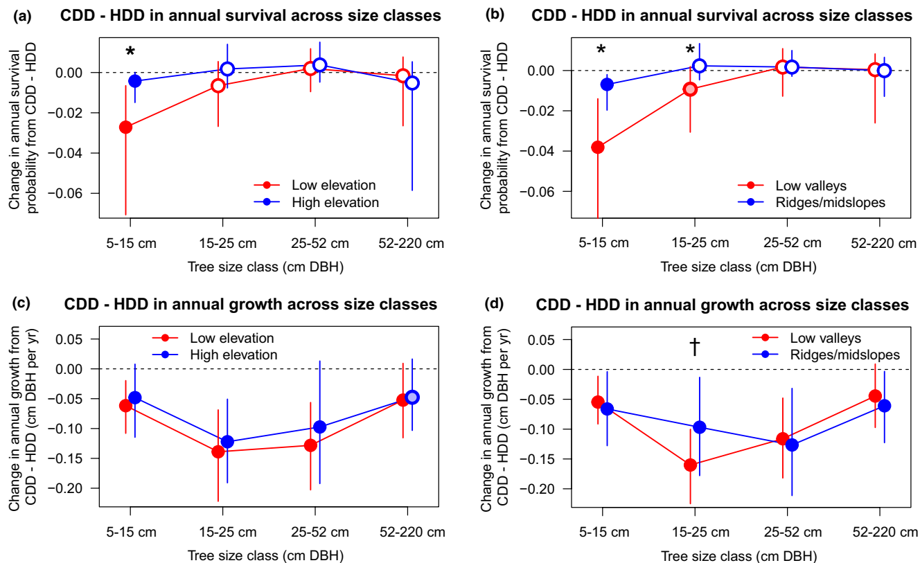
FIGURE 3 Average-predictive comparisons of CDD–HDD in survival (a and b) and growth (c and d) across tree size classes. (a) Differences in CDD–HDD in survival across size classes at high (1,450 m) and low (450 m) elevations. (b) Differences in CDD–HDD in survival between forest plots with lower values of PC2_{MinSpring} , indicative of lower elevation valley bottoms that experience colder minimum spring temperatures associated with greater relative humidity, and forest plots with higher values of PC2_{MinSpring} , indicative of low-elevation ridges and higher elevation midslopes/ridges that experience warmer minimum spring temperatures associated with lower relative humidity (Figures S1 and S3). (c) Differences in CDD–HDD in growth across size classes at high (1,450 m) and low (450 m) elevations. (d) Differences in CDD–HDD in growth between forest plots with lower values of PC2_{MeanSummer} , indicative of lower elevation valley bottoms that experience colder mean summer temperatures associated with greater relative humidity, and forest plots with higher values of PC2_{MeanSummer} , indicative of low-elevation ridges and higher elevation midslopes/ridges that experience warmer mean summer temperatures associated with lower relative humidity (Figures S1 and S3). Solid-filled values have \geq 95\% probability of being different from zero, lightly filled points have a 90%–95% probability of being different from zero, and open points have a < 90\% probability of being different from zero. Error bars reflect 95% credible intervals. Stars indicate highly probable differences ( \geq 95\% ), and crosses indicate probable differences (90%–95%) across elevations or PC2 (i.e. difference between red and blue values)
