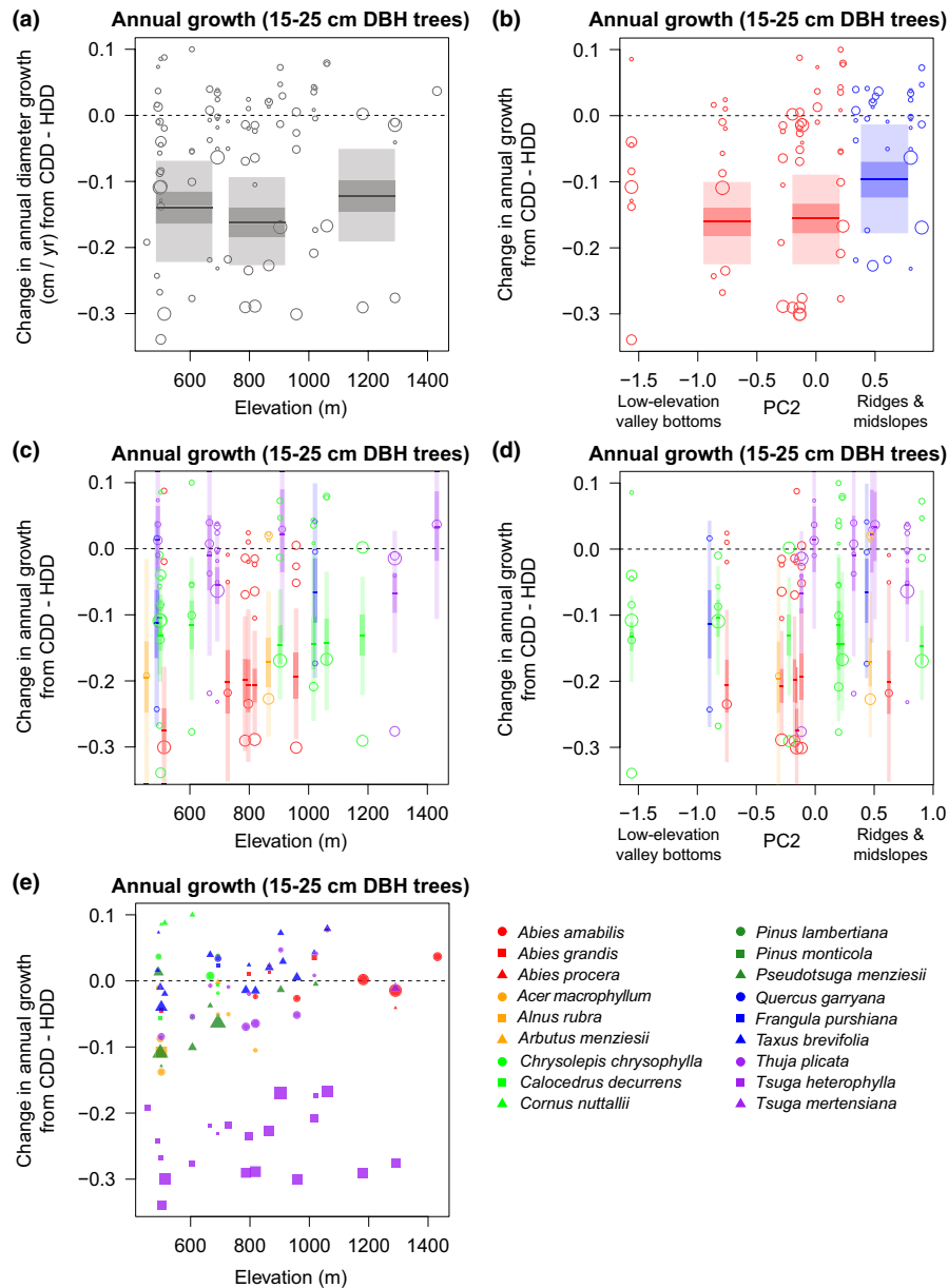
FIGURE 6 Average-predictive comparisons of CDD–HDD in growth of 15–25 cm DBH trees across elevation and microclimate variables ( PC2_{\text{MeanSummer}} ). CDD–HDD in growth was defined as the difference in annual diameter growth rate (cm per year) for a focal tree in a stand of conspecific trees (at mean tree density) versus in a stand of heterospecific trees (at mean tree density). See Figure 4 for description of panel details; all panel details here are the same as in Figure 4, except data here are for growth of 15–25 cm DBH trees and PC2 is PC2_{\text{MeanSummer}} . The red and blue colours in panel B indicate a 90.8% and 89.1% probability that CDD–HDD in growth was more negative at low and intermediate values of PC2_{\text{MeanSummer}} , respectively, than at high values of PC2_{\text{MeanSummer}} (as opposed to colours in panels (a) and (b) in Figures 4 and 5, which indicate a \geq 95\% probability of difference between groups)
