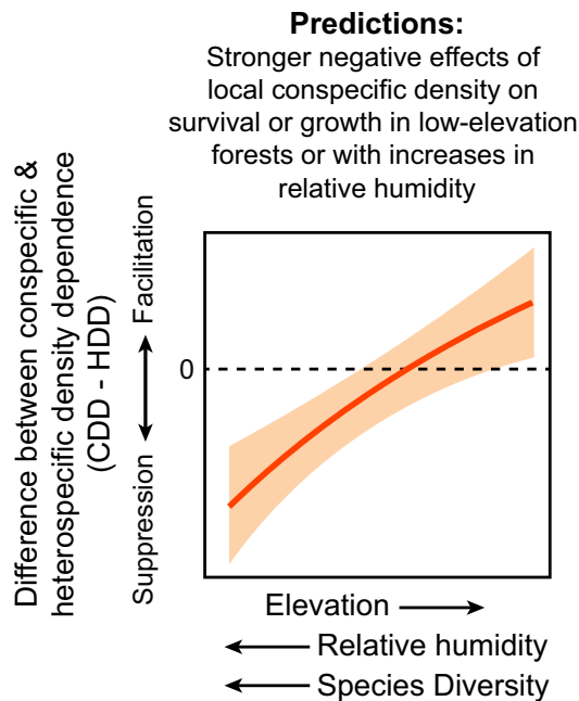
FIGURE 1 Key predictions evaluated in this study, which are generated from the hypothesis that increases in relative humidity associated with elevation alter interactions among plants and their host-specific enemies/mutualists and generate stronger negative effects of conspecific density on survival and growth. CDD–HDD is measured as the effect of local conspecifics on survival or growth (i.e. CDD) minus the effect of local heterospecifics (i.e. HDD; Comita et al., 2010; Hülsmann et al., 2020; LaManna, Mangan, et al., 2017). Mean CDD–HDD across species (orange line) is predicted to be stronger in lower elevation forests associated with greater relative humidity and greater tree species diversity. Negative CDD–HDD is generated by intraspecific competition or interactions with host-specific natural enemies. Disease risk is greater and growing seasons longer at lower elevations which may generate negative CDD–HDD by favouring host-specific pathogens. At higher elevations, freezing temperatures, lower humidity, greater seasonality, more precipitation falling as snow and lower nutrient availability may generate neutral or positive CDD–HDD by reducing pathogen loads and favouring host-specific mutualists
