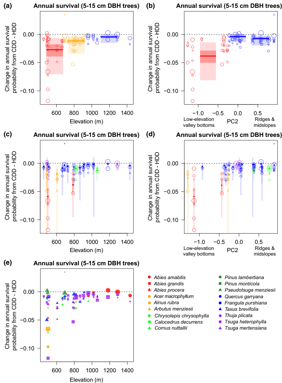
FIGURE 4 Average-predictive comparisons of CDD–HDD in survival of 5–15 cm DBH trees across elevation and microclimate variables. CDD–HDD in survival was defined as the difference in annual survival probability for a focal tree in a stand of conspecific trees (at mean tree density) versus in a stand of heterospecific trees (at mean tree density). (a and b) Average-predictive comparisons were calculated across forest plots at low, intermediate and high values of elevation (a) and PC2_{\text{MinSpring}} (b) using a Bayesian bootstrap approach to make inference to other forest plots within each group (see text for details). (c and d) Average-predictive comparisons were also calculated at the forest-plot level to show probable differences among the forest plots used in this study. (a–d) Average-predictive values for each species-by-plot combination (circles) are sized according to their sample size (number of individuals). Median values (dark strip), 50% credible intervals (i.e. interquartile range; darker bar) and 95% credible intervals (lighter bar) of the group- or plot-level average-predictive values are also shown. (a and b) Red groups have \geq 95\% probability of difference from blue groups; orange group has \geq 90\% probability of difference from blue groups. (c and d) Colours indicate highly probable differences ( \geq 95\% probability of difference) among forest plots (red = lower than \geq 5 plots; orange = lower than \geq 1 plot; grey = no differences from other plots; green = lower than \geq 1 plot and higher than \geq 1 plot; blue = higher than \geq 1 plot; purple = higher than \geq 5 plots). (e) Average-predictive values for each species-by-plot combination across elevations
